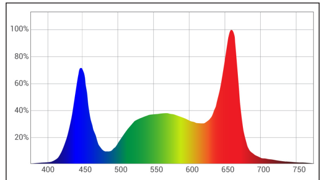
X6 - This full spectrum maximizes red and blue nm wavelengths to allow for optimal chlorophyll A and B absorption with a balance of green wavelengths to allow much deeper canopy penetration.
