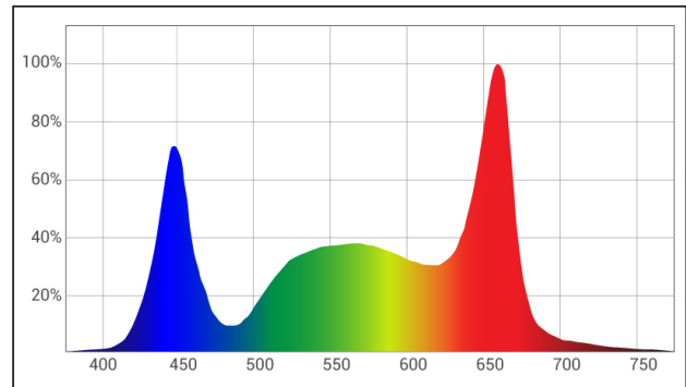
X6 - This full spectrum maximizes red and blue nm wavelengths to allow for optimal chlorophyll A and B absorption with a balance of green wavelengths to allow much deeper canopy penetration.
