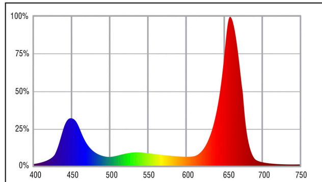
F3 - This spectrum is known as the full cycle spectrum developed specifically to foster quality growth at each stage. It produces fast germination and high quality vegetative and flowering plants.
